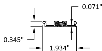
10 FLAT FILLER
