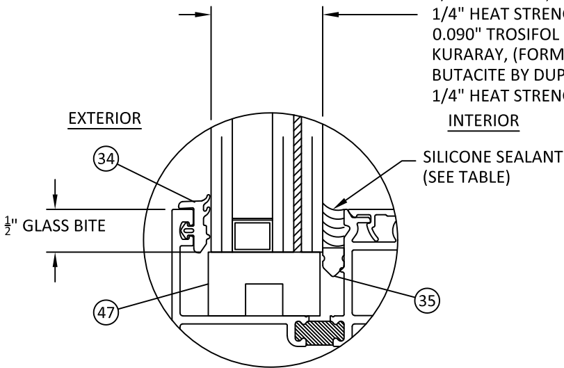
GLAZING DETAIL C (WET GLAZED)
