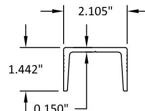
17 RECEPTOR ANCHOR
