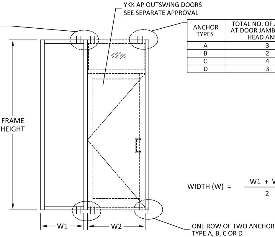
SINGLE DOOR WITH TRANSOM
