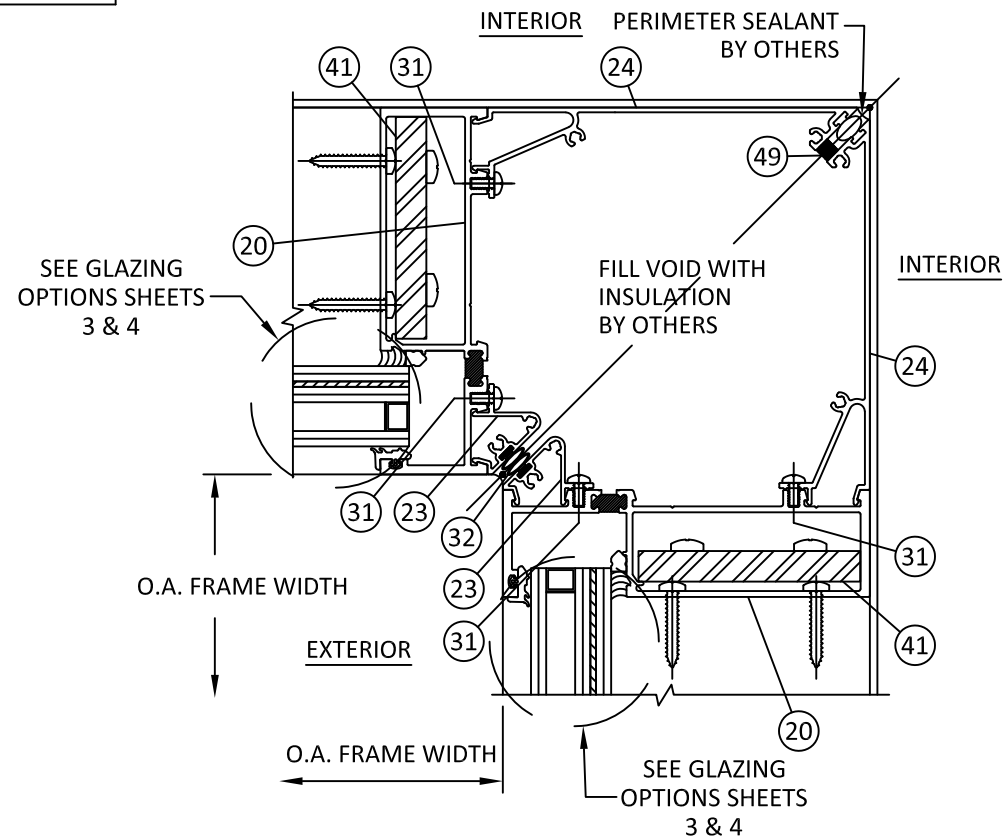
P 15 HORIZONTAL SECTION 90° INSIDE CORNER STANDARD CONFIGURATION
