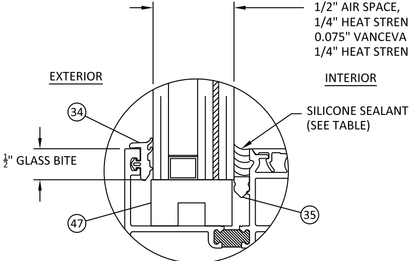
GLAZING DETAIL B (WET GLAZED)
