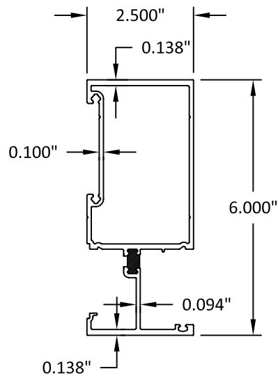
2 HEAVY DUTY JAMB MULLION
