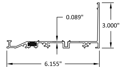
9 SILL FLASHING
