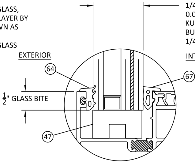
GLAZING DETAIL D (DRY GLAZED) S.M.I. ONLY
