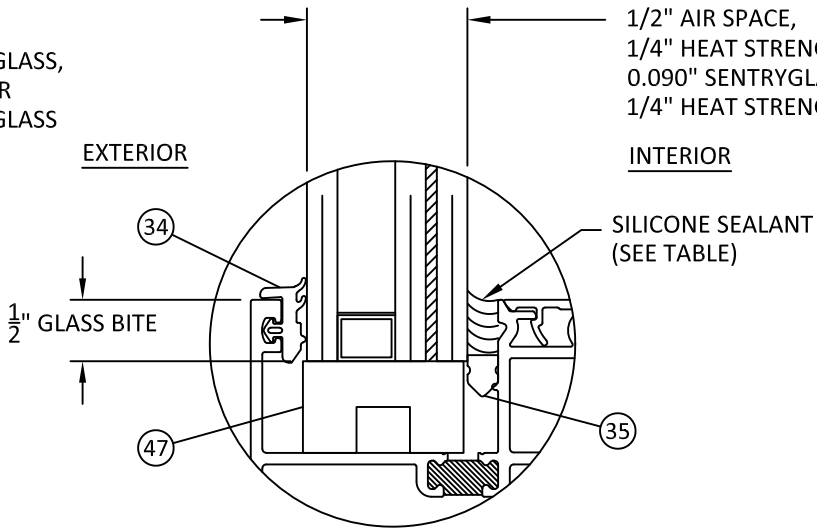
GLAZING DETAIL A (WET GLAZED)
