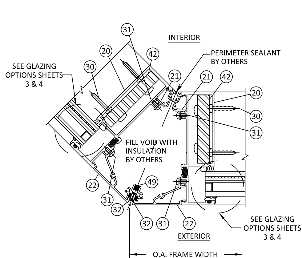
M 15 HORIZONTAL SECTION 135° OUTSIDE CORNER STANDARD CONFIGURATION
