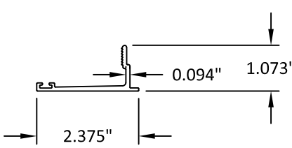
51 RECEPTOR SNAP COVER
